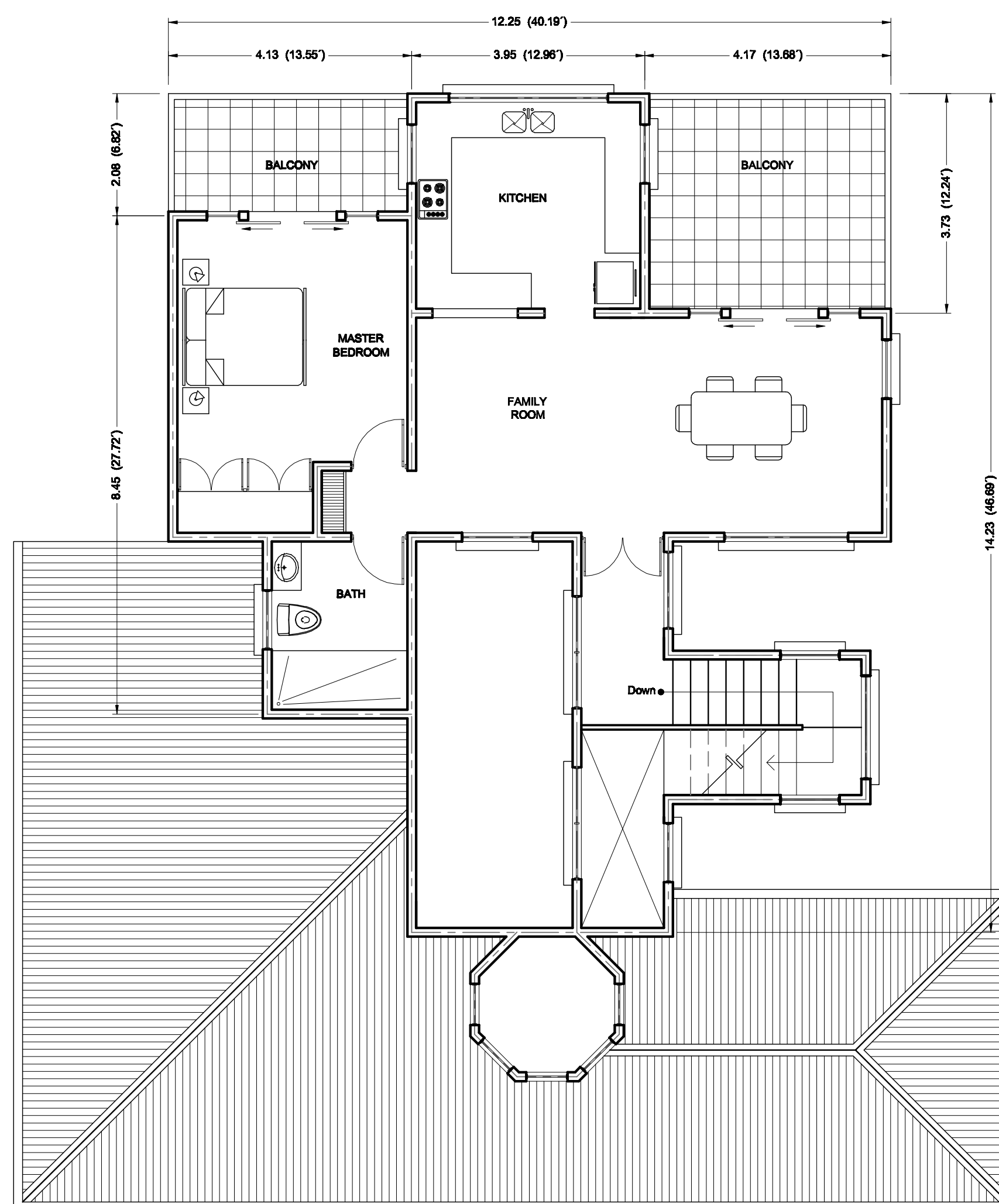
GUANACASTE SECOND FLOOR SCALE: 1:75
