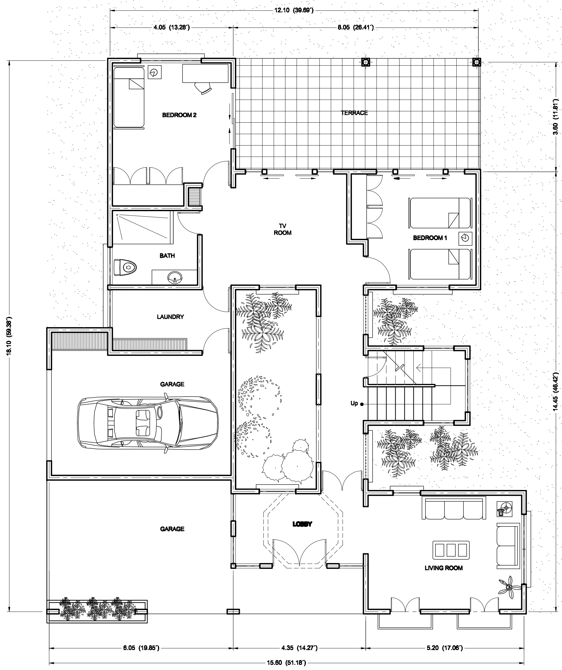
GUANACASTE FIRST FLOOR SCALE: 1:75
